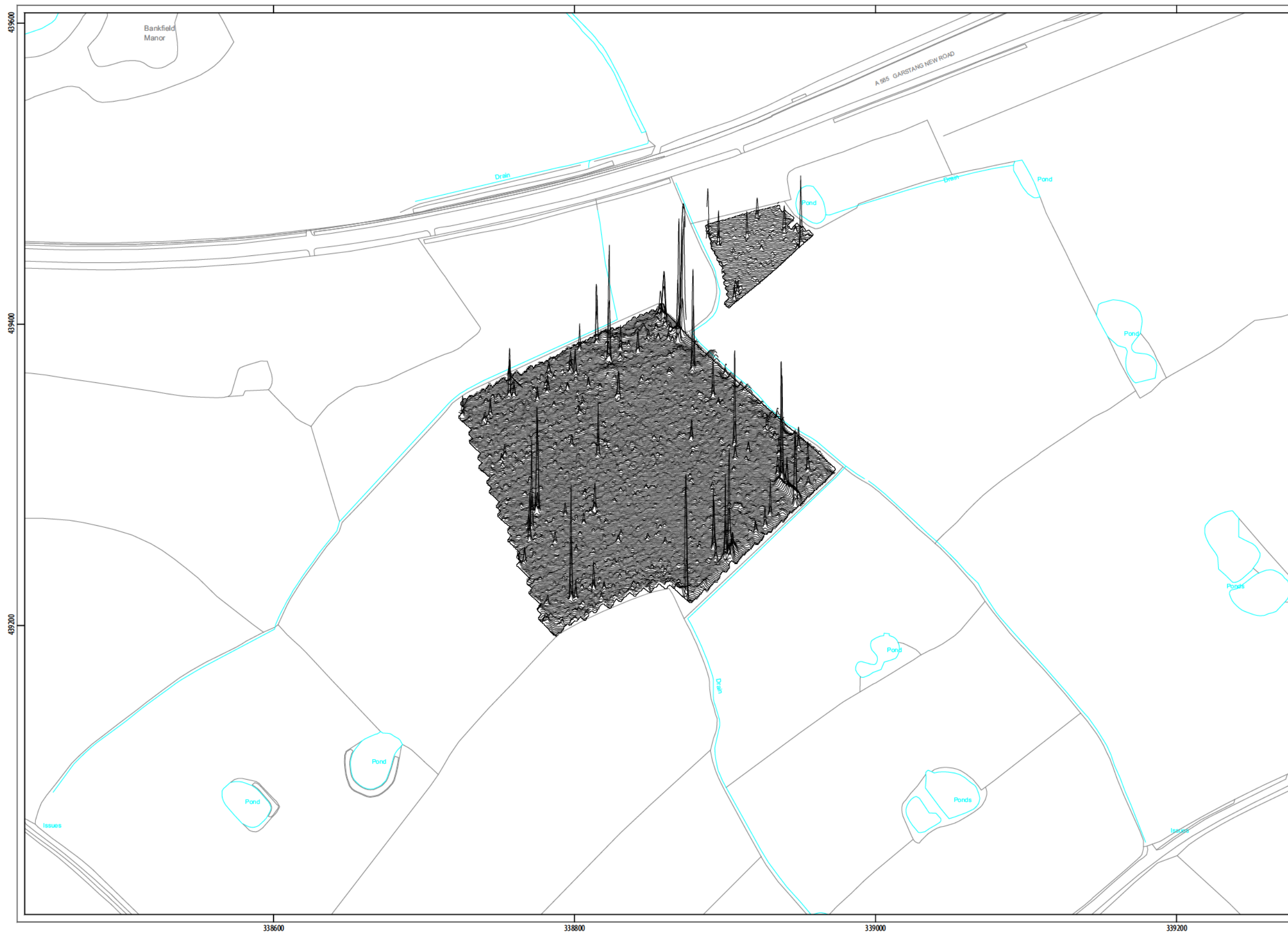
ILLUS 23 XY trace plot of minimally processed magnetometer data; Sector 5 (1:2,500)
